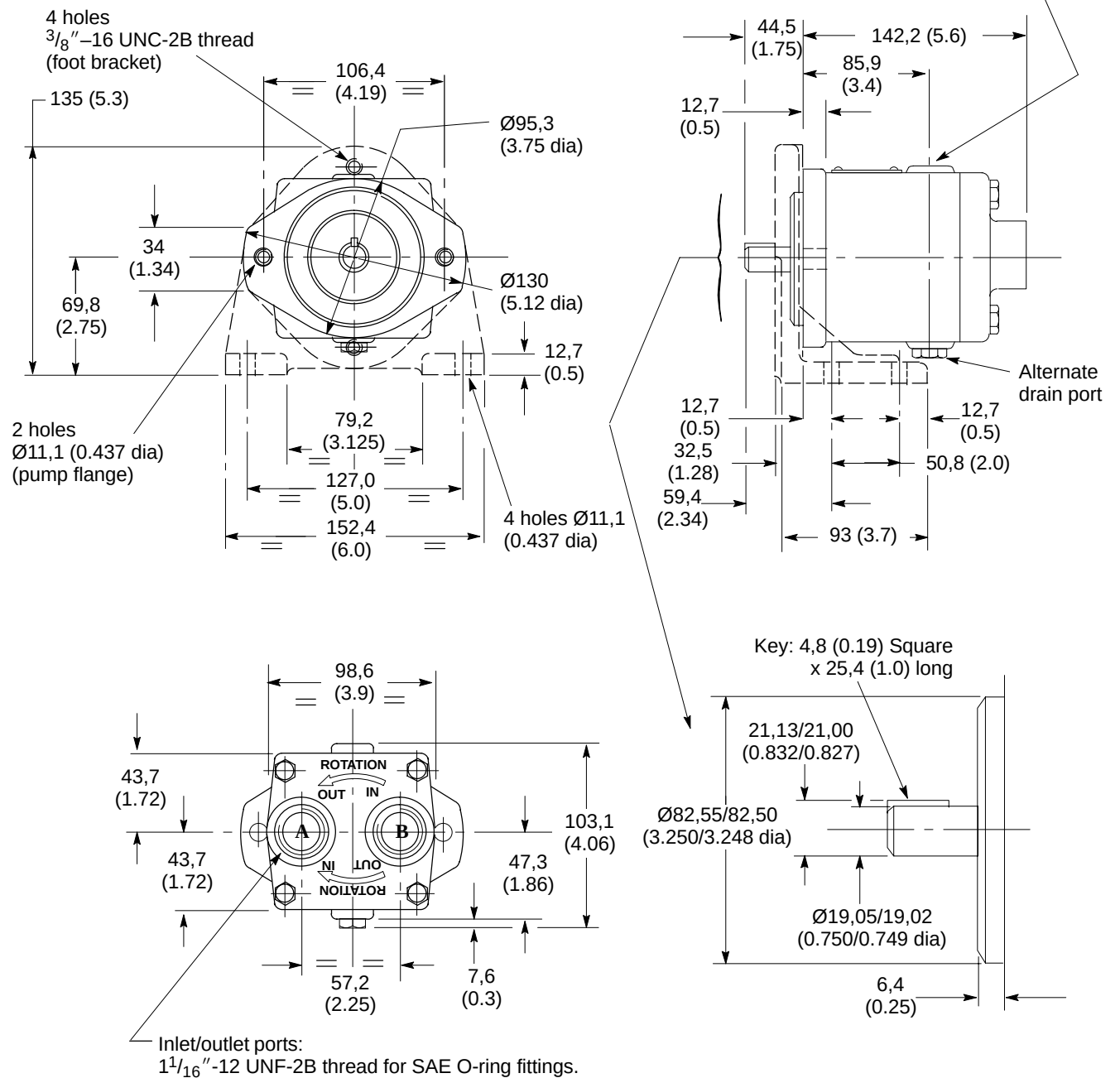
Detail of shaft, key and locating diameter
