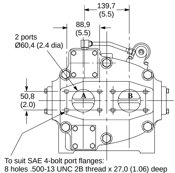
View on rear end of pump
